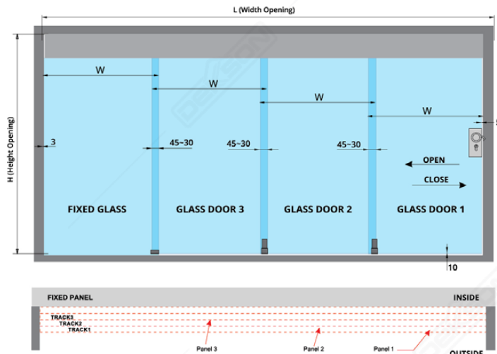
DOOR PANEL TRACK 4M SGT 4100 (3+1) NA (2 pcs)
