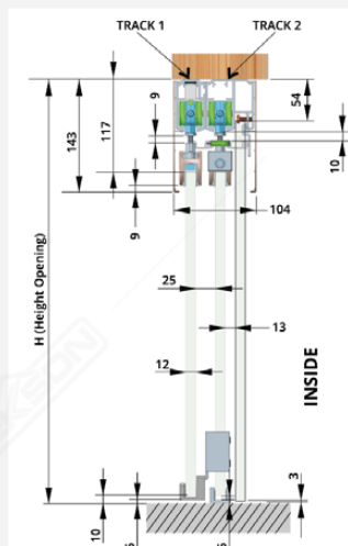
FIX PANEL TRACK 3M SGT 3100 (2+1) NA (1 pc)
