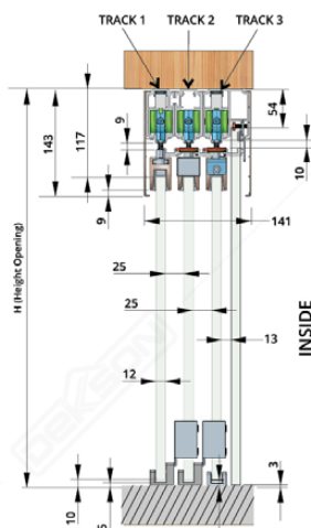
FIX PANEL TRACK 4M SGT 4100 (3+1) NA (1 pc)
