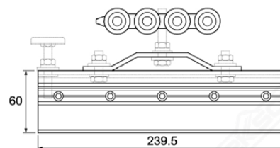
FLOOR GUIDE INSET 12 MM (1 pc)
