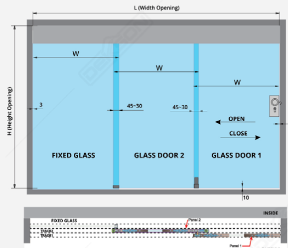
DOOR PANEL TRACK 3M SGT 3100 (2+1) NA (2 pcs)
